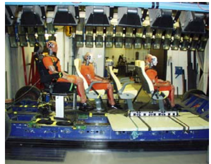
Wavemaster and Voyager at the test-setup
